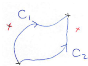
図 21: \int_{C_1} f(z) dz = \int_{C_2} f(z) dz
