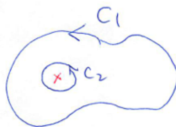
図 22: \int_{C_1} f(z) dz = \int_{C_2} f(z) dz
