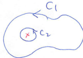
図 26: \int_{C_1} f(z) dz = \int_{C_2} f(z) dz
