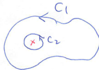
図 12: \int_{C_1} f(z) dz = \int_{C_2} f(z) dz
