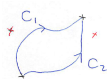
図 25: \int_{C_1} f(z) dz = \int_{C_2} f(z) dz
