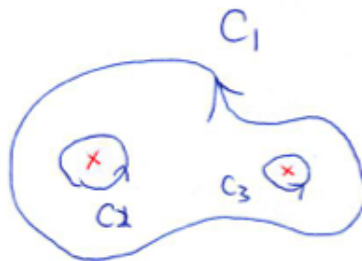
図 27: 応用: \int_{C_1} f(z) dz = \int_{C_2} f(z) dz + \int_{C_3} f(z) dz
