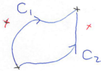
図 11: \int_{C_1} f(z) dz = \int_{C_2} f(z) dz
