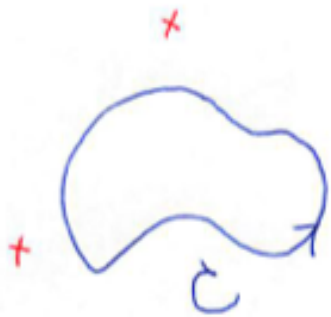
図 23: \int_C f(z) dz = 0
