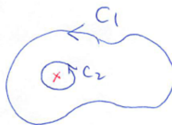
図 13: \int_{C_1} f(z) dz = \int_{C_2} f(z) dz
