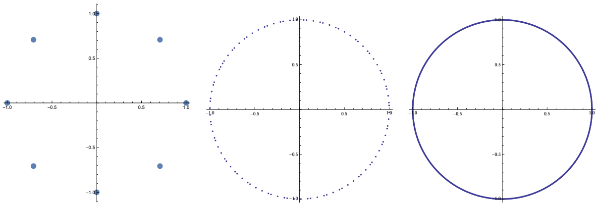
図 5: p(1, 1/8) , p(1, \sqrt{2}) ( 1 \leq n \leq 100 の 100 個), p(1, \sqrt{2}) ( 1 \leq n \leq 1000 の 1000 個)
